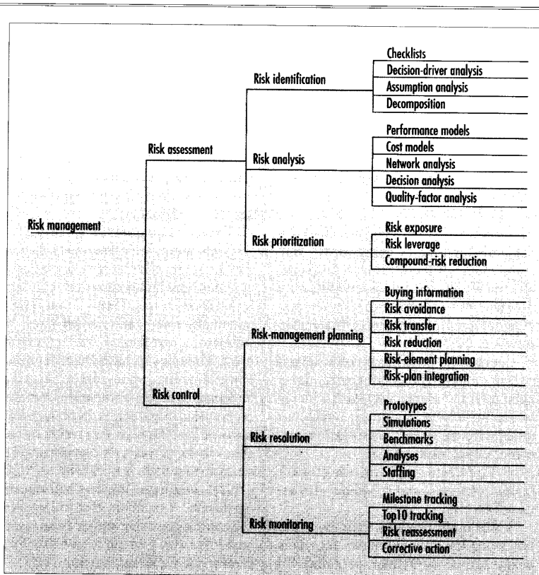
FIGURE 2. SOFTWARE RISK MANAGEMENT STEPS.
